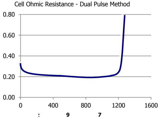
9 Typical Characteristics to 0.8 Volts
